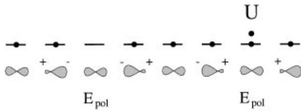
FIG. 2. Schematical representation of the excited SDW state. The charge excitation defining the effective Coulomb repulsion U and induced polarizations are indicated.
